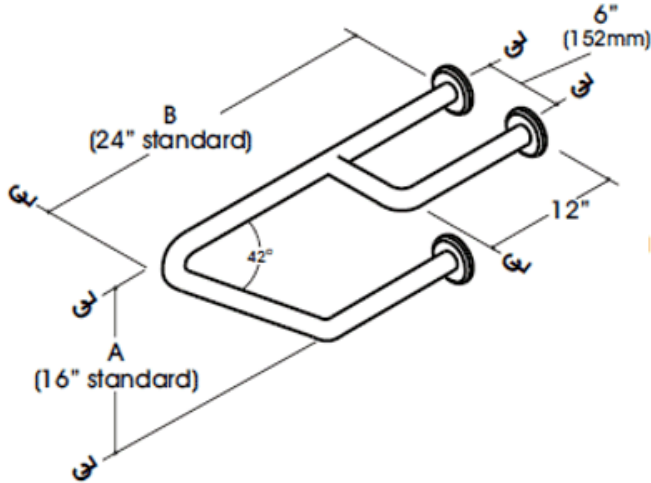
18 Side Bar c/w outrigger
