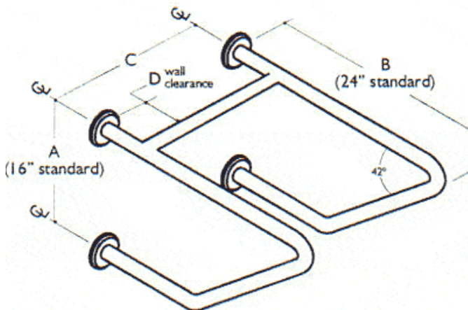
21 Toilet Straddle Bar
