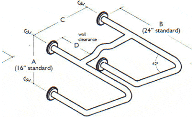
22 Toilet Straddle Bar for flush valve
