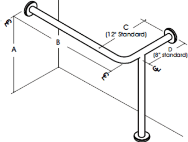
38 Single Floor Support
