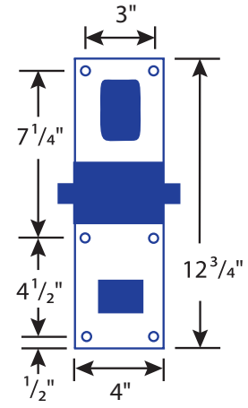
Mounting Bracket (support removed for clarity)
